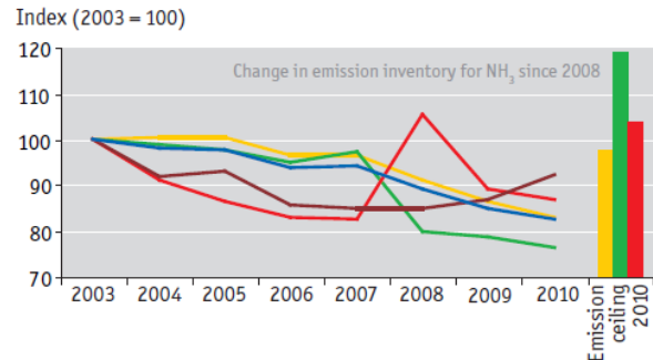
Chart 1 → Development of emissions of primary particulate matter and secondary particulate matter precursors in the Czech Republic, 2003–2010 and the national emission ceilings (for NO x , SO 2 and NH 3 ) for 2010 [index, 2003 = 100]*
