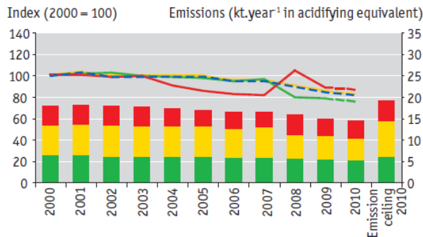
Chart 1 → Total emissions of acidifying substances in the Czech Republic, 2000–2010 and the level of national emission ceilings for 2010 [index, 2000 = 100]; [kt.year -1 in acidifying equivalent]*
