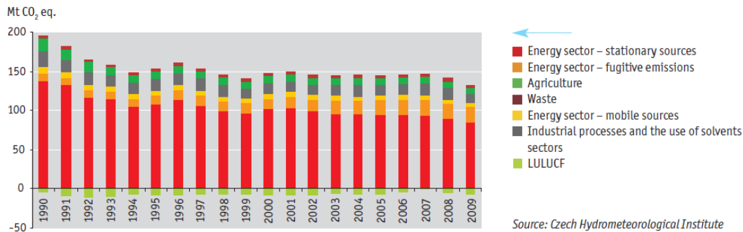
Chart 1 → Development of greenhouse gas emissions by sector in the Czech Republic [Mt CO 2 eq.], 1990–2009
